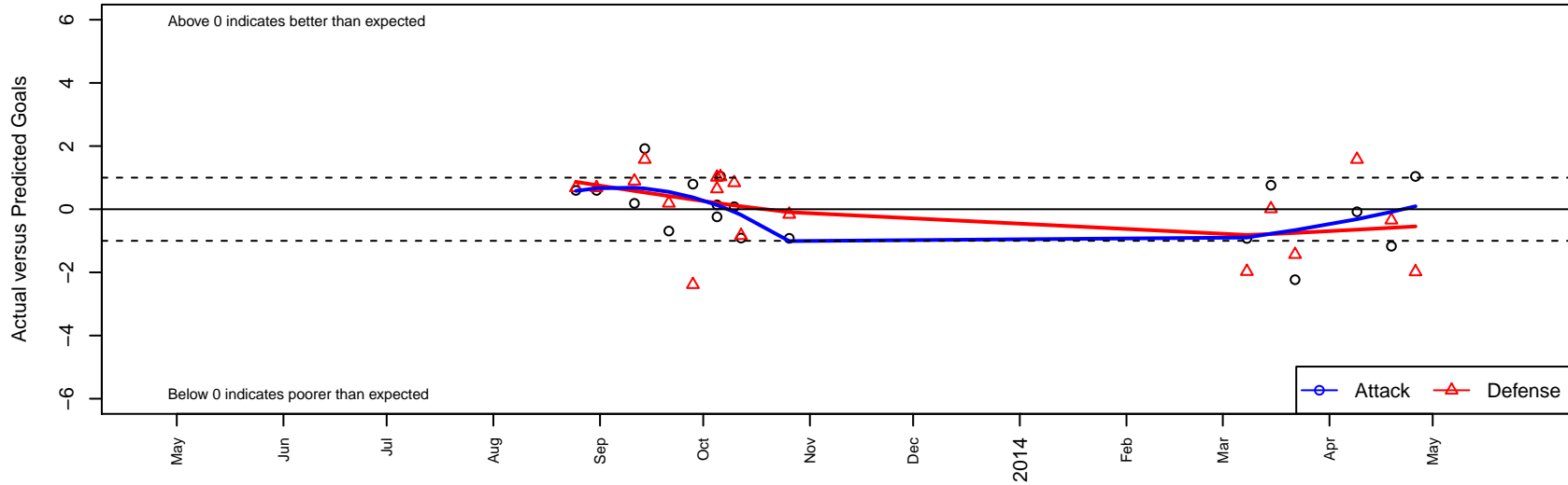
Soccer Xpress Atomic Black G99 Dots are actual minus expected GF (blue circles) and GA (red triangles). Blue line is smoothed change in attack strength. Red is smoothed change in defense strength.
